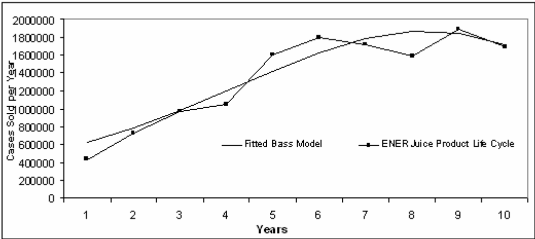
Figure 1: Estimated Bass Model from ENER Juice Data
